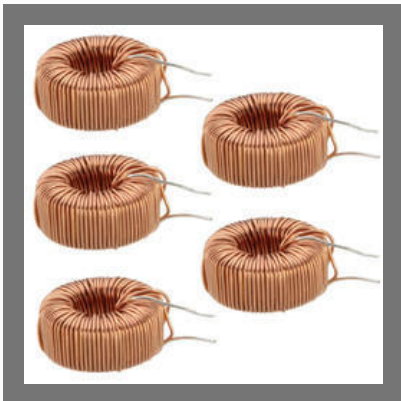
Common Mode Choke Coil
